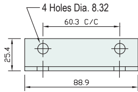
Mounting Bracket Detail
