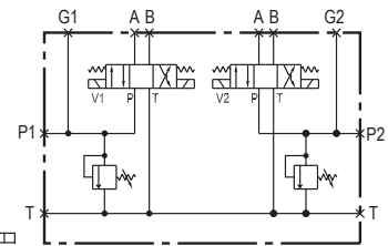
Manifold Circuit (Shown With Relief Option)
