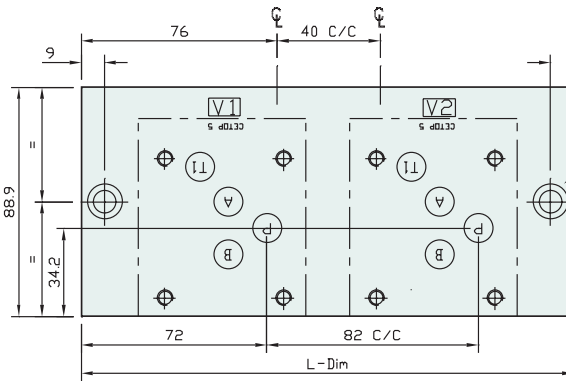
Relief Valve Cavity
