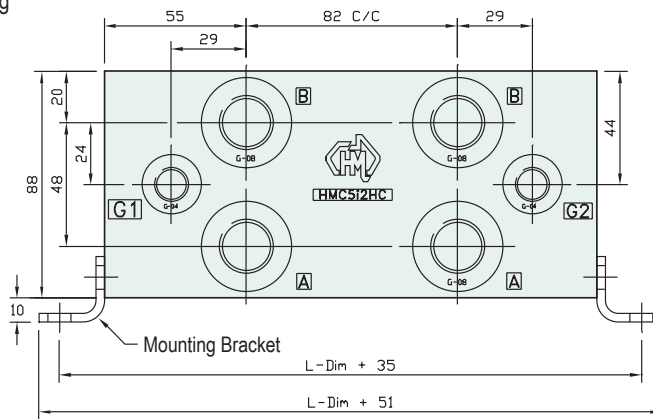
Mounting Bracket Detail
