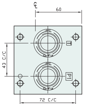
Relief Valve Cavity
